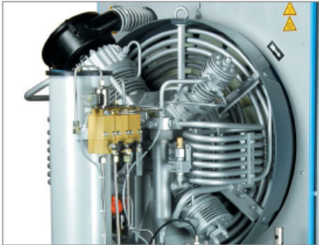
4-stage high pressure compressor block K 150
